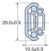
Cross sections
