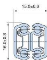
Cross sections
