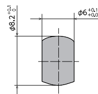
<Recommended dimensions for mounting a rotating shaft>
