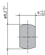
<Recommended dimensions for mounting a rotating shaft>
